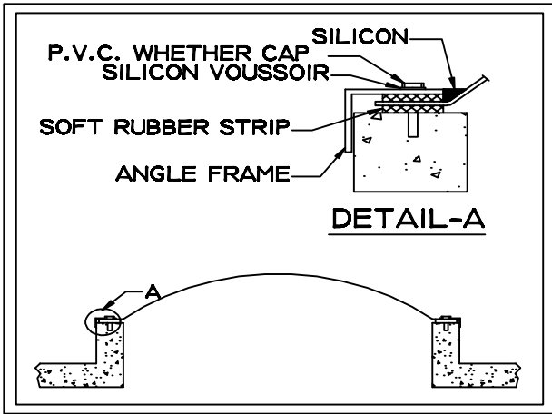
FLAT FLANGE
