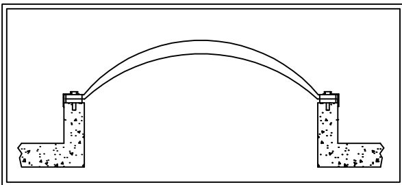
DOUBLE SKIN
